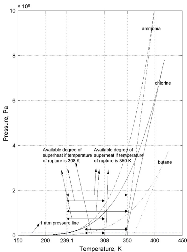
Fig. 1. Pressure–temperature curves and superheat limit loci for ammonia, chlorine, and butane, showing degrees of superheat at different stages of container rupture.
