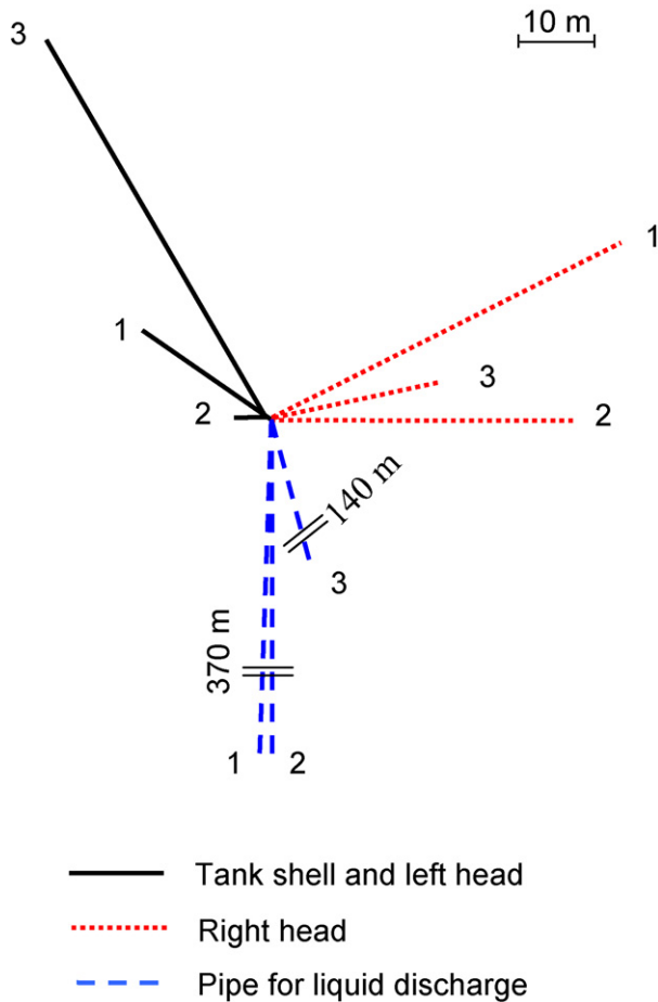
Fig. 3. Schematic view of the direction of flight and range of fragments of three vessels – nos. 1–3 – after a BLEVE. Source: Drawn from the data of Schulz-Forberg et al. [80].
