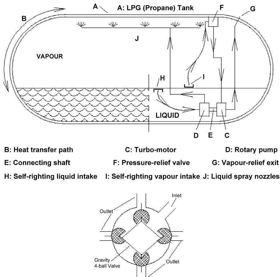
Fig. 5. The 'anti-BLEVE safety system' patented by Young [113].
